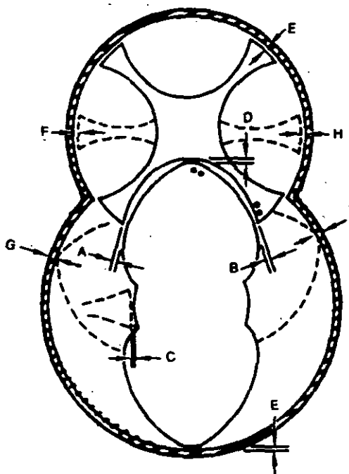
Figure 1. Location of Blower Clearance Check Points
