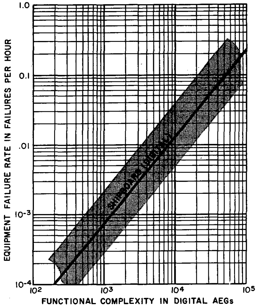
Figure 2003.2. Failure-Rate Estimation Chart for Digital Electronic Functions.
